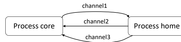
Figure 3. Communication channels between processes in the Promela model of the German cache coherence protocol
