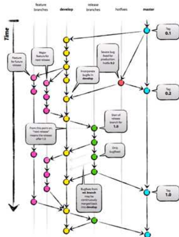
Fig. 6. General git-flow diagram
