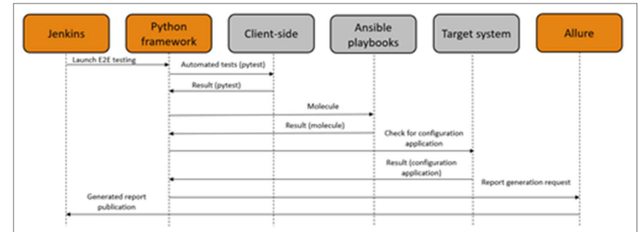
Fig. 4. UML sequence diagram
