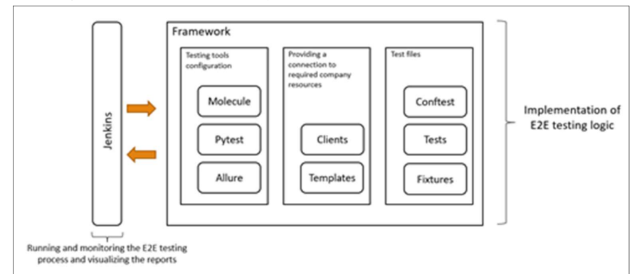
Fig. 5. High-level design of the developed software
