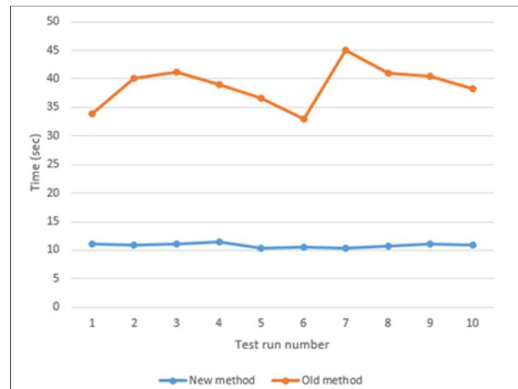
Fig. 8. Results of the first experiment
